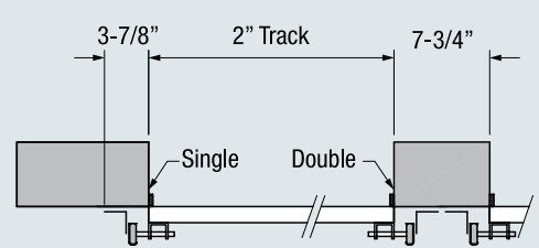
Bracket Mounted Track
