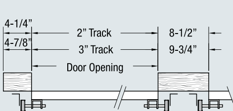
Continuous Angle Track Wood Jambs
