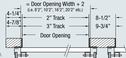
Reverse Angle Track Steel / Masonry Jambs
